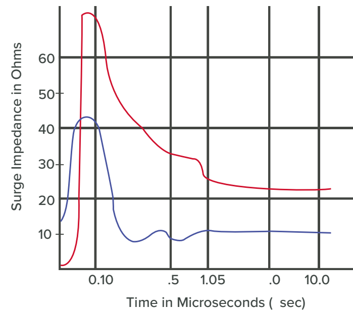
Figure 2: Surge Impedance
